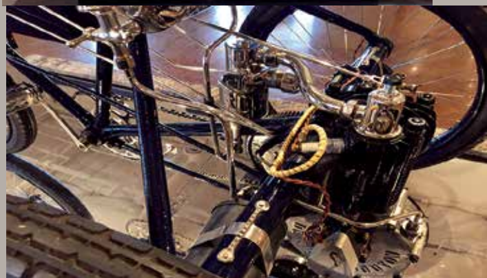
Peugeot Tricycle 2-1/4 HP 1899 Powered by the famous De Dion Bouton single cylinder engine, this late 19th century Peugeot was painstakingly restored in Holland by Gilbert Warming. This testament to the pioneer days of motorcycling is exceedingly rare and genuine, retaining many of the original components, notably including its De Dion engine and Peugeot two-speed gearbox.
